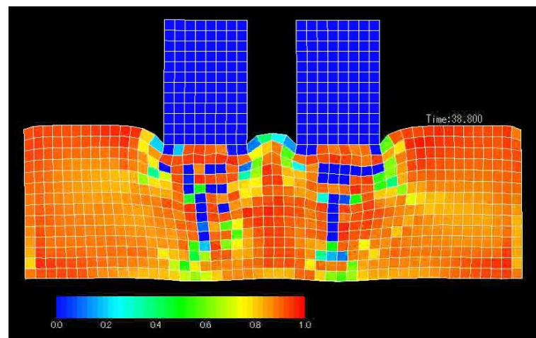
Fig② With adjacent foundation (separate a part)
