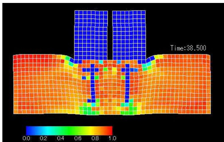
Fig③ With adjacent foundation (closely spaced)
